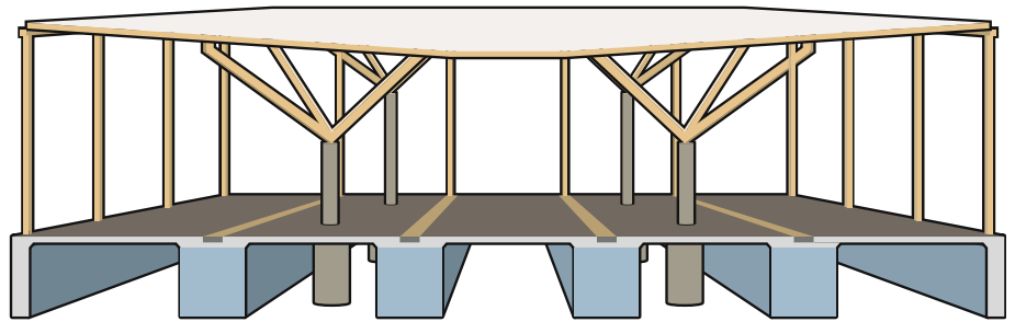
A simplified cross-section through a classroom module showing the four internal columns sitting on piles between the tanks. The tanks shown are an early iteration, but the principle is close to the as-built version.
